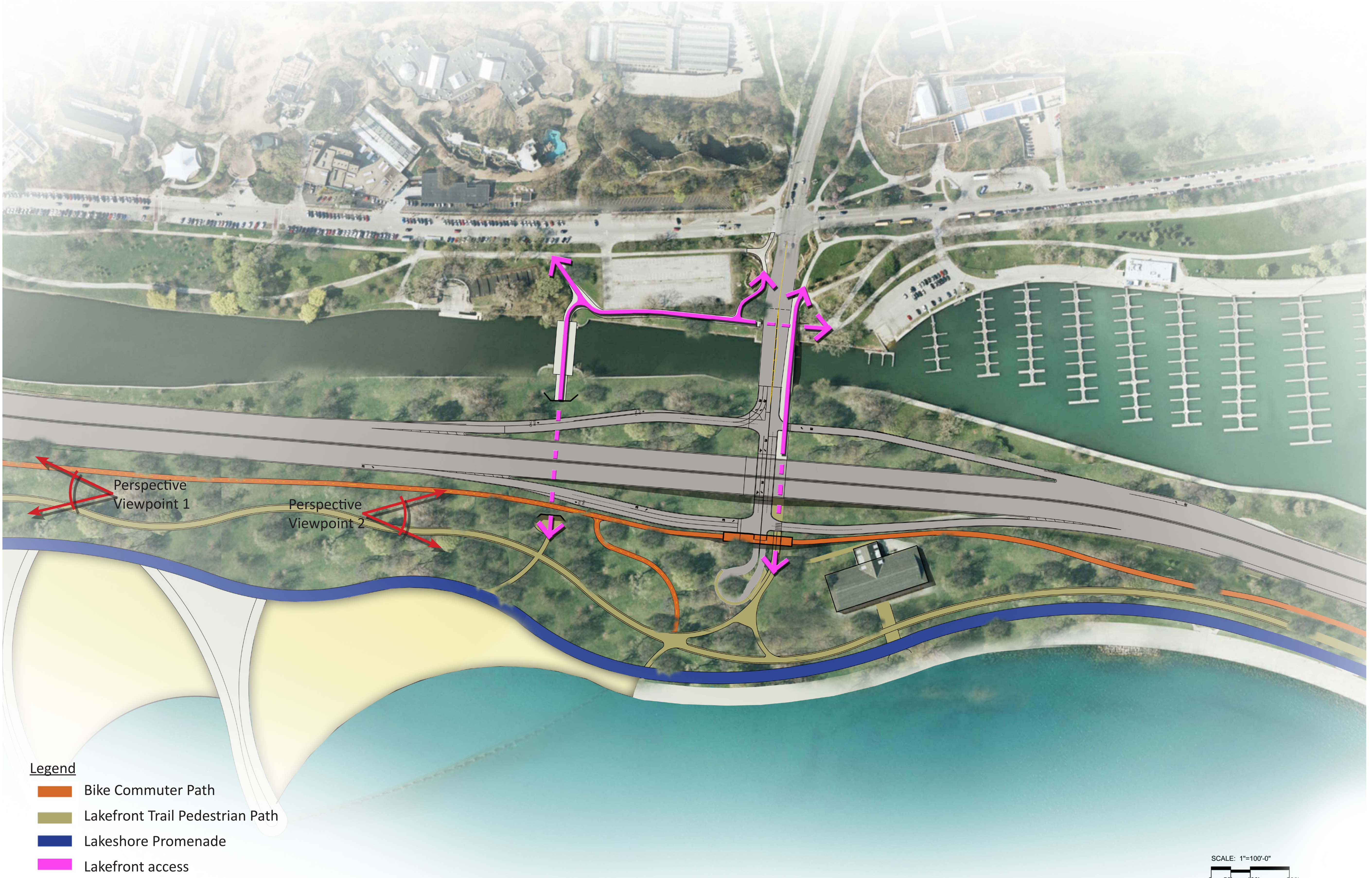
Plan View
